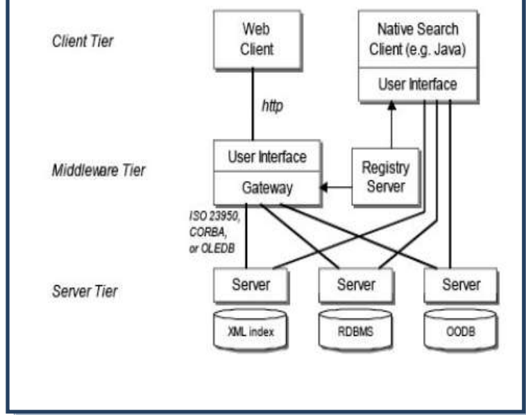
Figure 8.4: Implementation View of Distributed Catalogue Services
