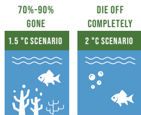
CORAL REEFS
