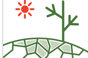
DROUGHTS
